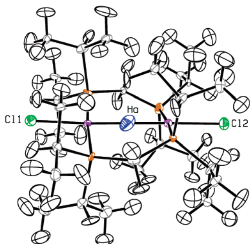
Figure 1. Anisotropic displacement ellipsoid view of 3 derived from neutron diffraction data at 40 K. All ellipsoids are shown at the 50% level. Selected bond lengths (Å): Ni1–Cl1, 2.250(6); Ni2–Cl2, 2.279(6); Ni1–H, 1.594(17); Ni2–H, 1.633(16); Ni1–Ni2, 3.227(5). Selected bond angles (deg): Ni1–H–Ni2, 177.5(11); Cl1–Ni1–P1, 91.65(27); Cl1–Ni1–H, 176.7(6).
